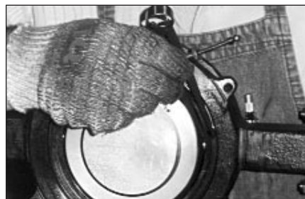
Figure 8 – Shows how to measure the gap between the body seat pocket ID and the disc OD.
